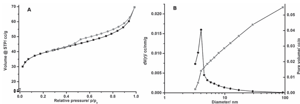
Figure 2. N 2 Adsorption (■)–desorption (○) isotherms of Al/Ni particles prepared by 50 min of sonication at 140 W cm −2 (A). BJH pore size distribution (●) and pore volume (■) of the same particles (B).
